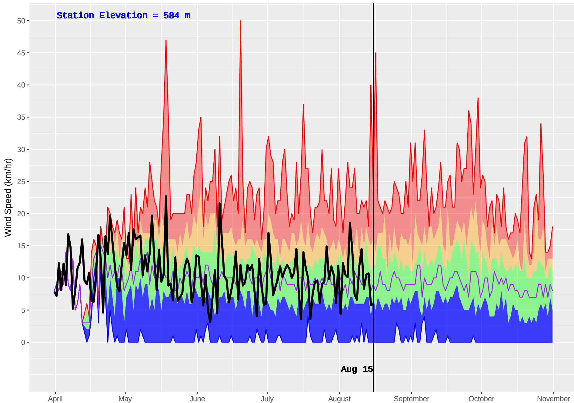
SIERRA (117) : Historical (1981–2016) and Current (2018) Daily Wind Speed
