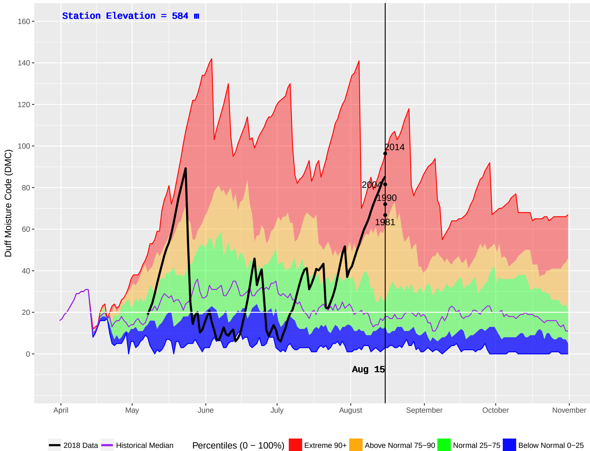
SIERRA (117) : Historical (1981–2016) and Current (2018) Daily Duff Moisture Code (DMC)
