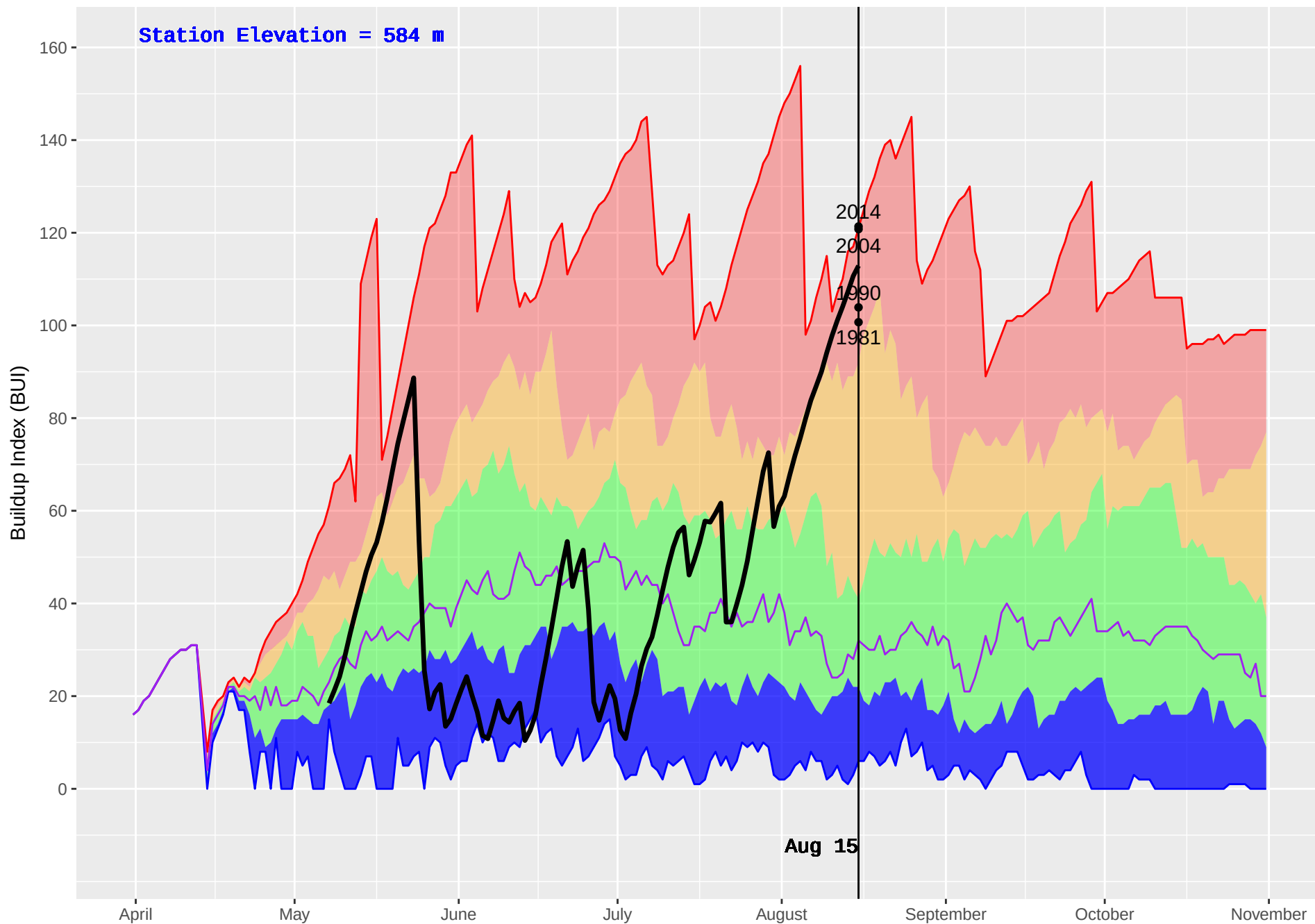
SIERRA (117) : Historical (1981–2016) and Current (2018) Daily Buildup Index (BUI)
